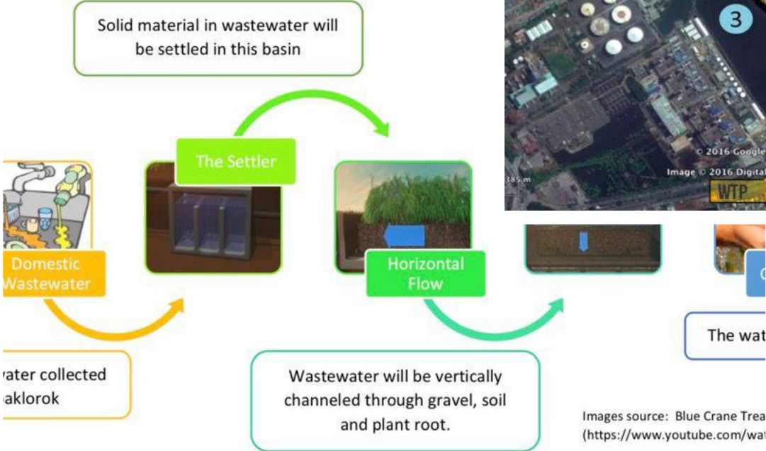
Figure 4 Green Wastewater Treatment System Schemes
